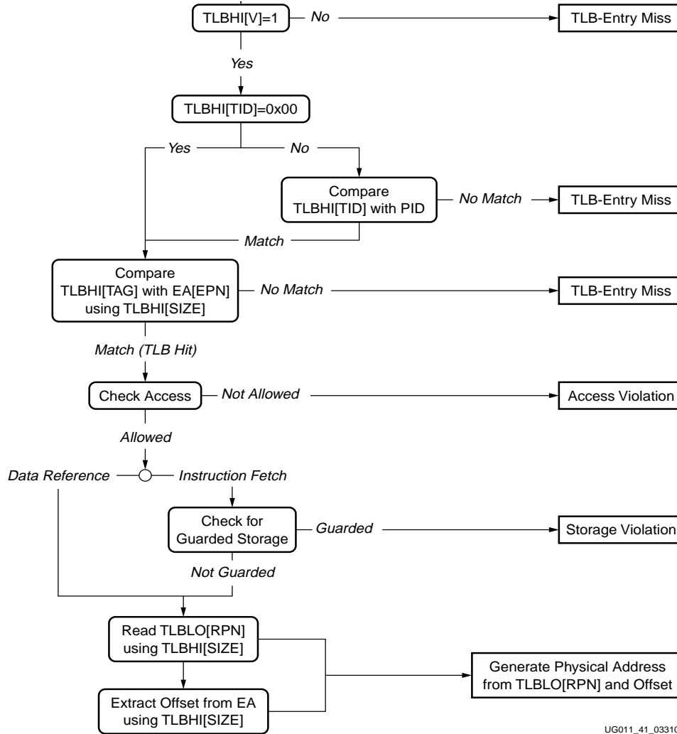
Figure 2-21: General Process for Examining a TLB Entry
