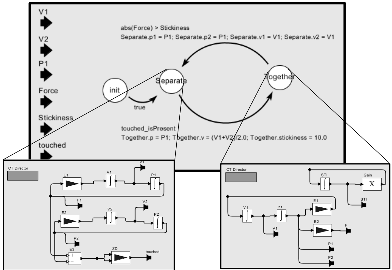
Figure 8. Hybrid system model in Ptolemy II, showing a hierarchical composition of a finite state machine (FSM) model and two continuous-time (CT) models. This example models a physical spring-mass system with two modes of operation. In the Separate mode, it has two masses on springs oscillating independently. In the Together mode, it the two masses are stuck together, and oscillate together with two springs. The model was created by Jie Liu and Xiaojun Liu.
